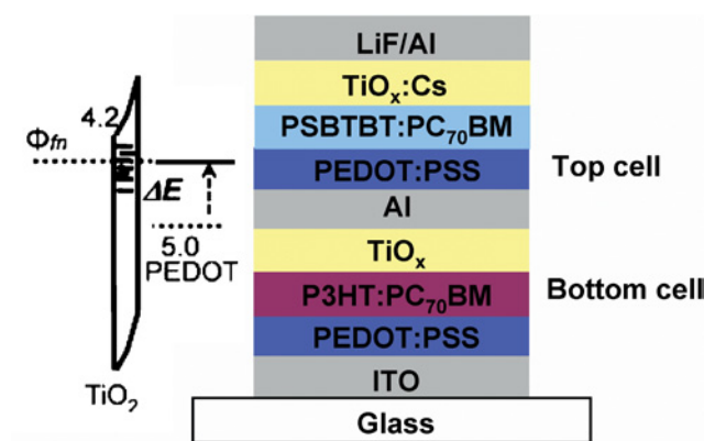
Figure 16. Schematic structure of tandem organic solar cell with TiO x based intermediate layers demonstrated by Sista et al. [84].
